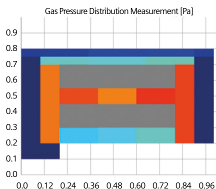
Figure 6: Static pressure measurement and simulation
