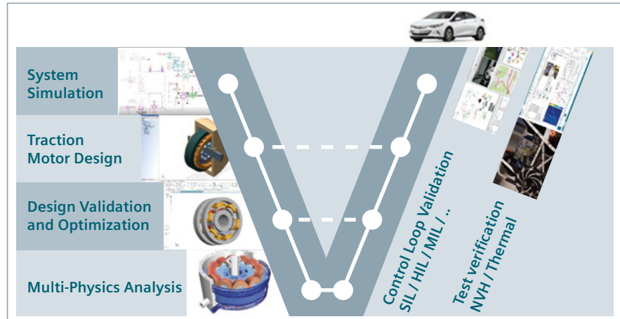
Figure 1: A typical traction motor design process V-cycle
