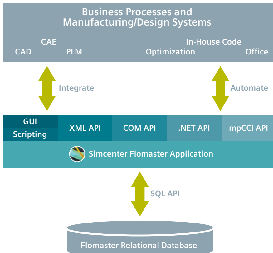
Figure 2: New approach integrating simulation and analysis with design
