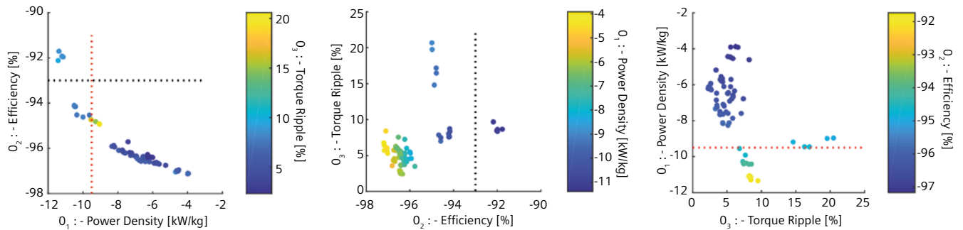
Figure 6: Pareto front projected onto different 2D surfaces. The dotted lines indicate design targets.
