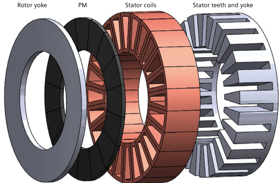
Figure 3: Exploded view of the single rotor AFPM
