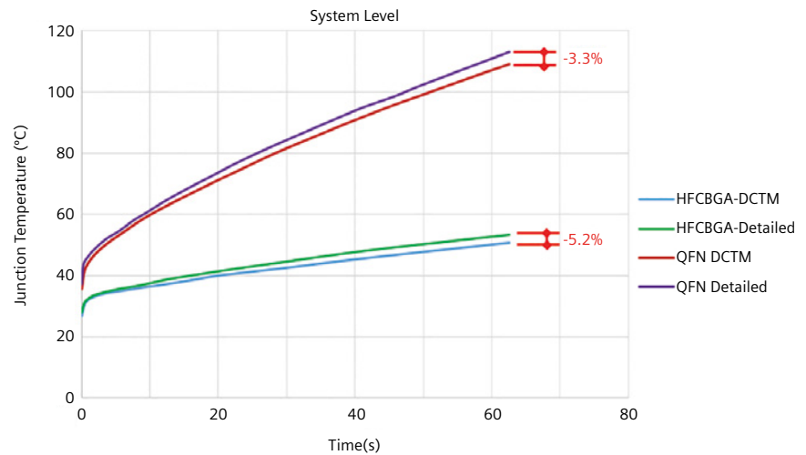
Figure 11: Transient response of detailed and dynamic compact thermal models of the QFN and HFCBGA packages in the AP Router
