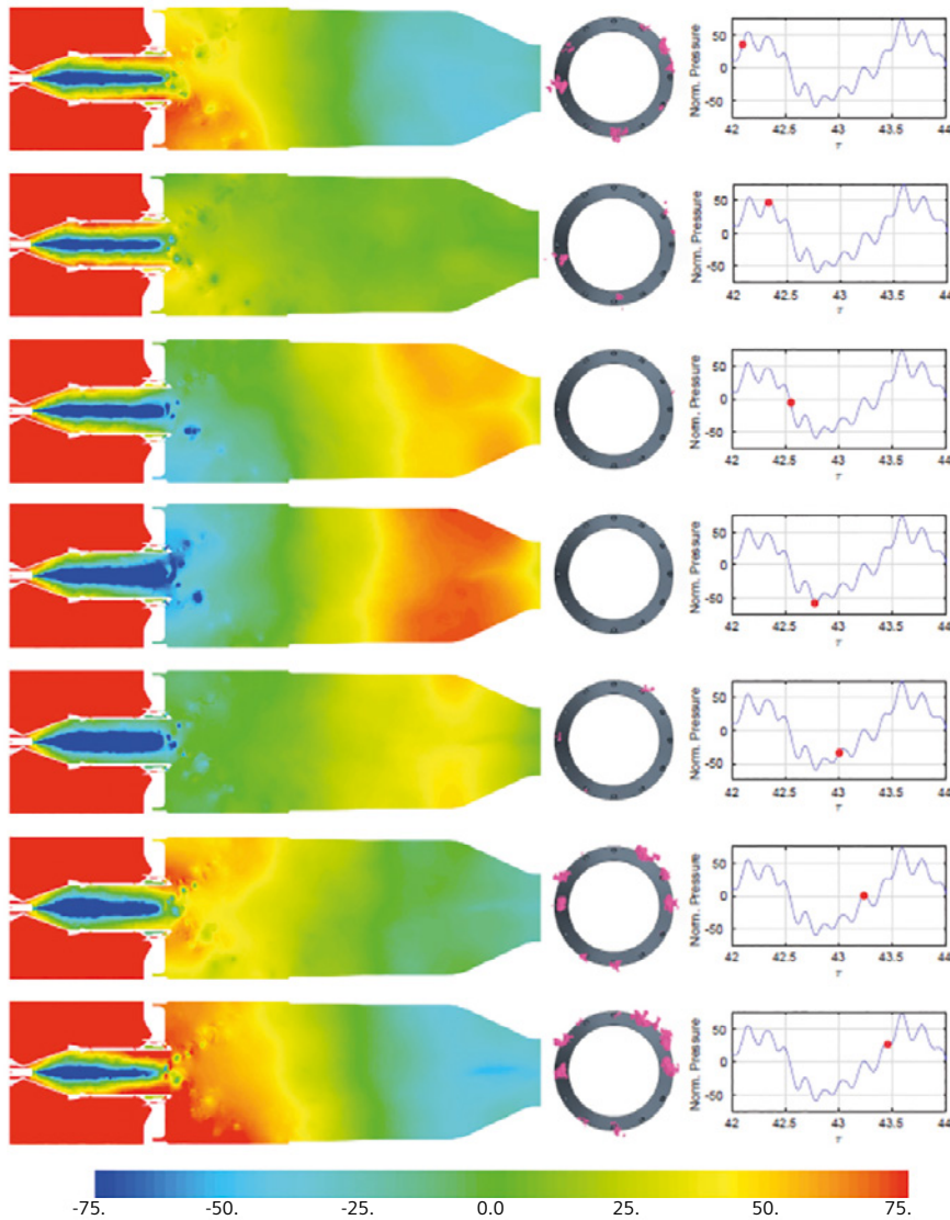
Figure 4: LES simulations of pure methane combustion
