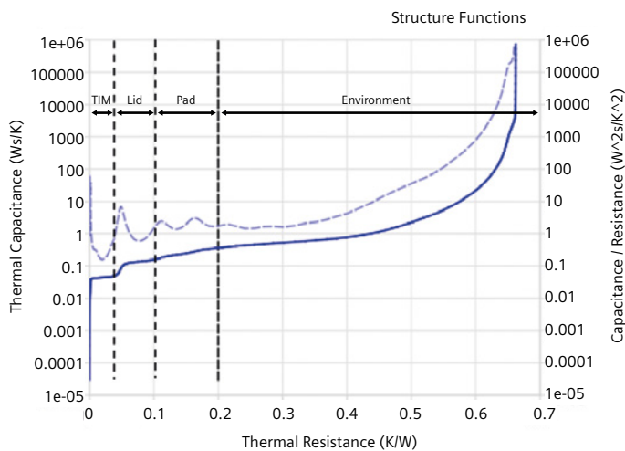
Figure 4a: Structure function curve for a HFCBGA package
