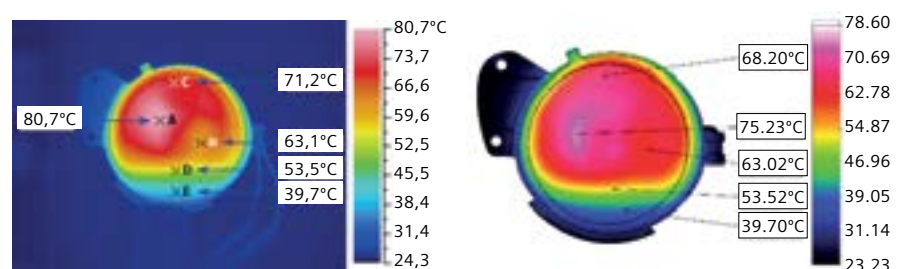
Figure 7: Thermography (left) and simulation (right)
