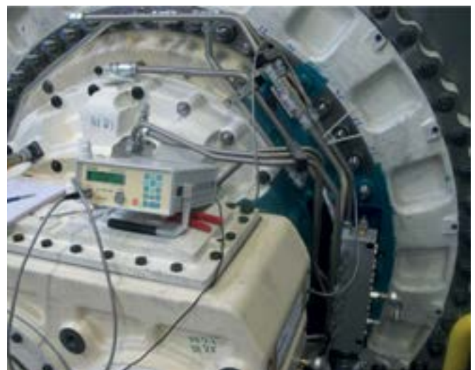
Figure 3. Flow meter verification testing
