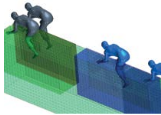
Figure 7: Bicycle pace-line drafting simulation: geometry and overset mesh setup in Simcenter STAR-CCM+.
